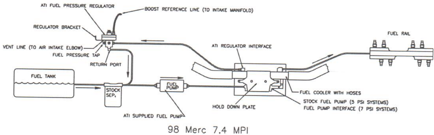
FIGURE G2 FUEL PUMP SCHEMATIC
