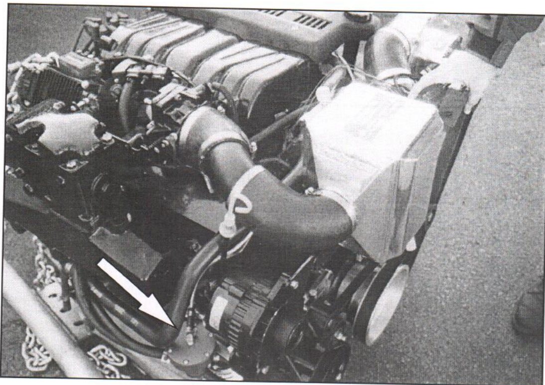
FIGURE G3 FUEL PRESSURE REGULATOR INSTALLATION
