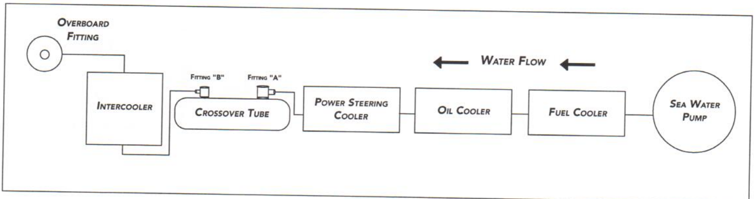
FIGURE F2 TYPICAL WATER ROUTING (NOTE: COOLER SEQUENCE WILL VARY BY BOAT)
