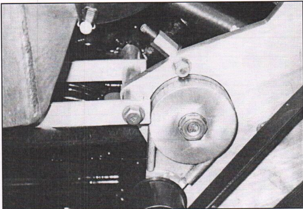
FIGURE D9 PORT SIDE INTERCOOLER TABS MOUNTED TO MAIN BRACKET AND HEAD
