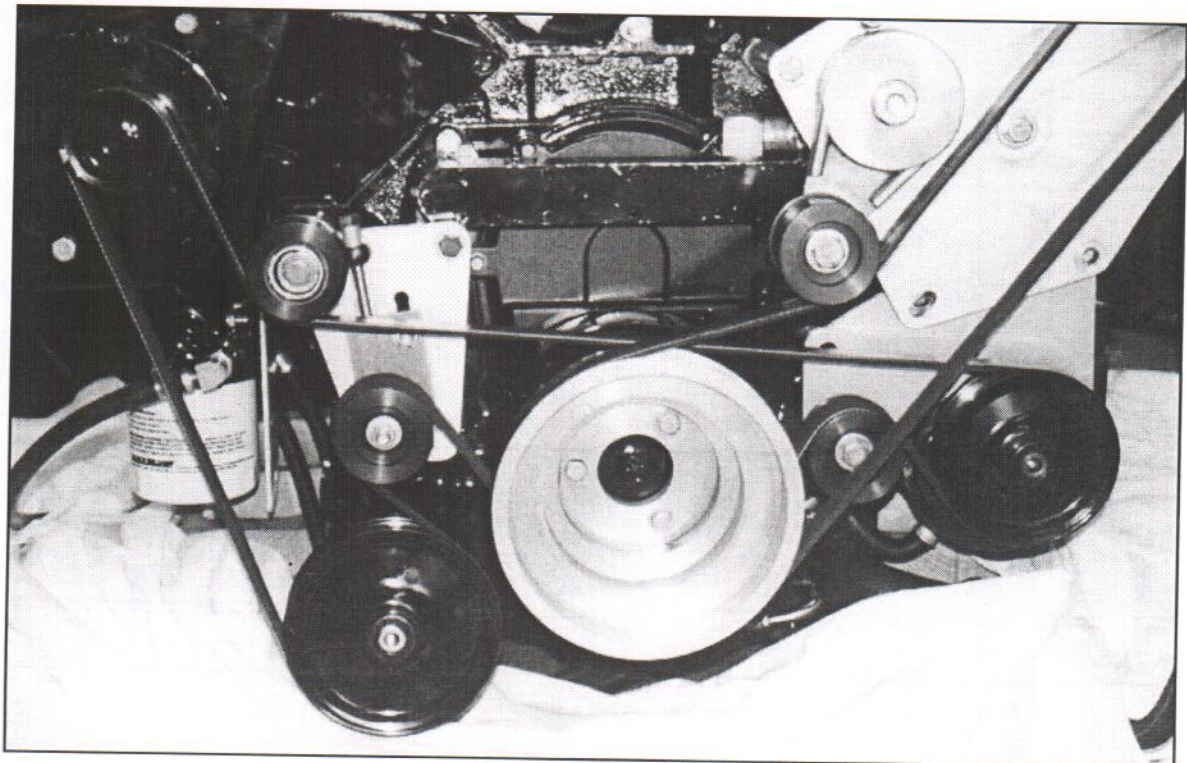
FIGURE D8 ACCESSORY BELT ROUTING
